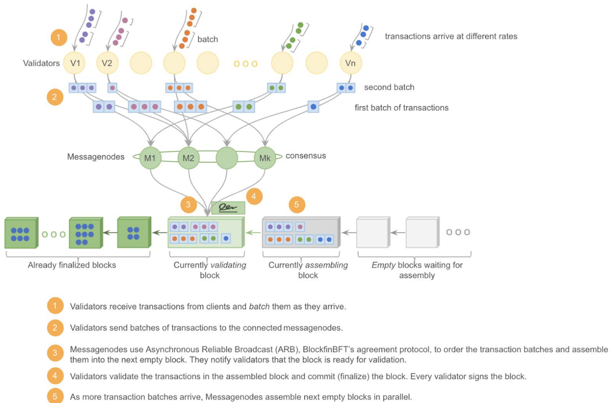
Fig. 3 — BlockfinBFT consensus steps
